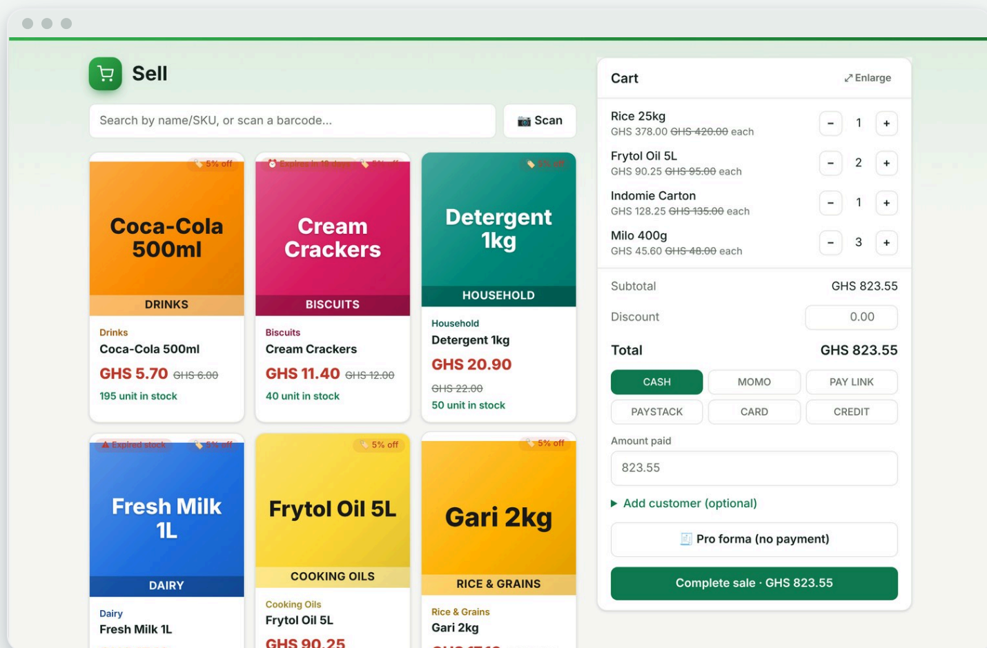
REAL SCREEN: THE TILL WITH A CART, DISCOUNTS AND PAYMENT BUTTONS
