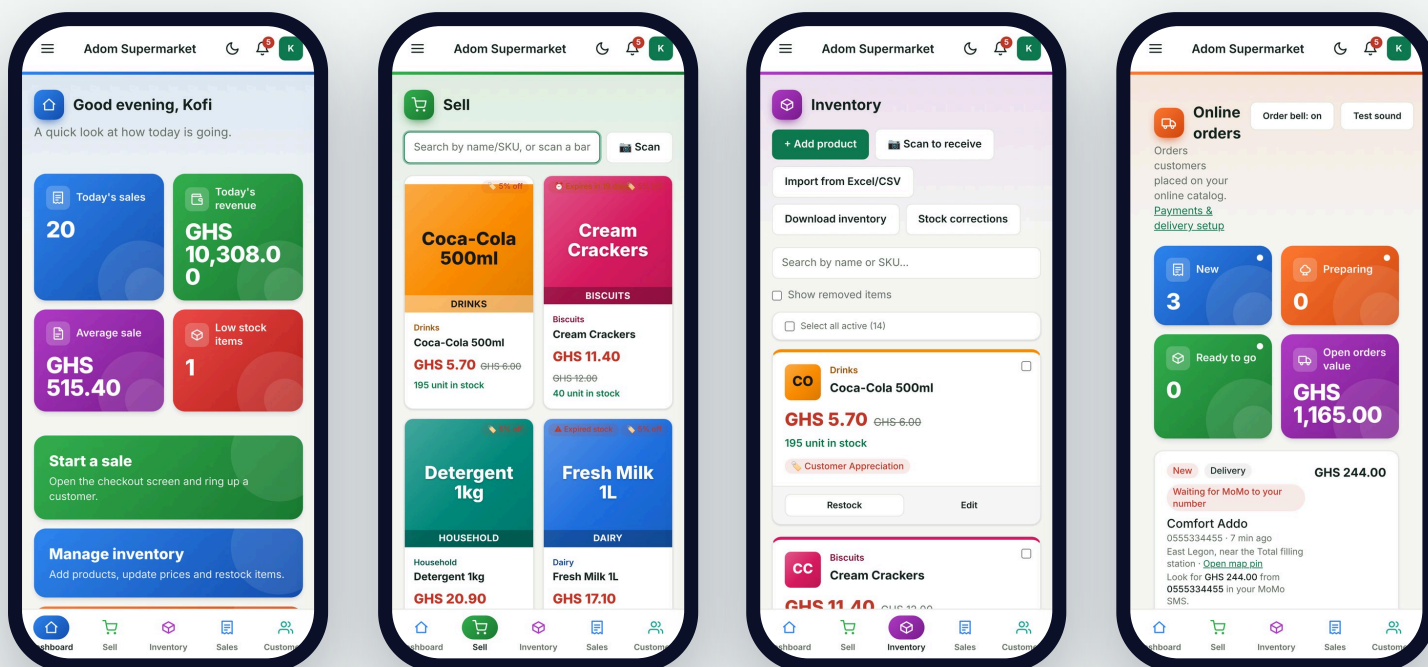
REAL SCREENS ON A PHONE: DASHBOARD, TILL, INVENTORY, ONLINE ORDERS
